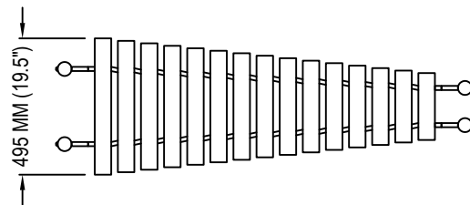
FRONT ELEVATION
