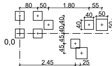
foundation plan check measurements on building site
