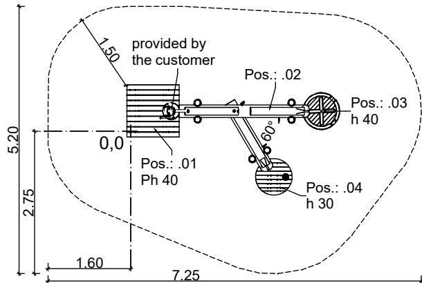
topview with minimum safety area
