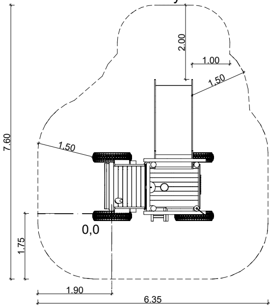
topview with minimum safety area
