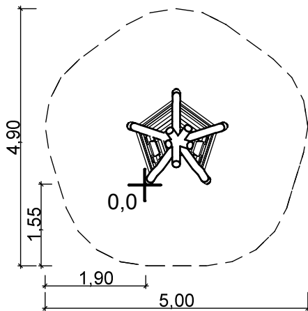
topview with minimum safety area
